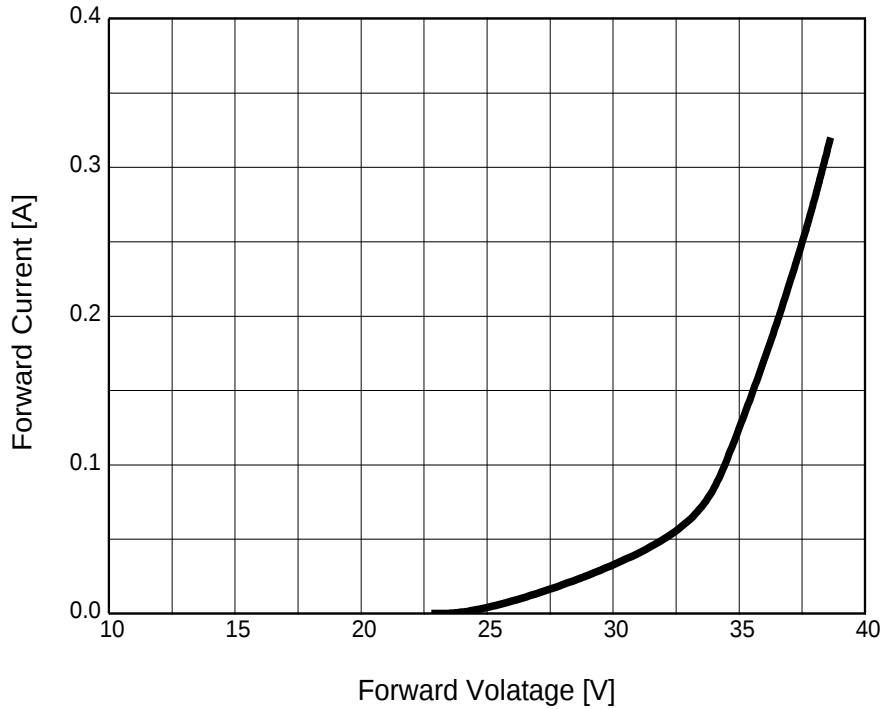
Fig 3. Forward Voltage vs. Forward Current , T_c = 25^\circ\text{C}
