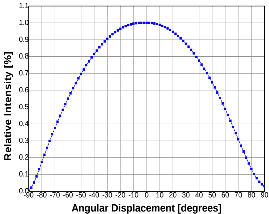
Fig 2. Radiant pattern, I_F = 180\text{mA}
