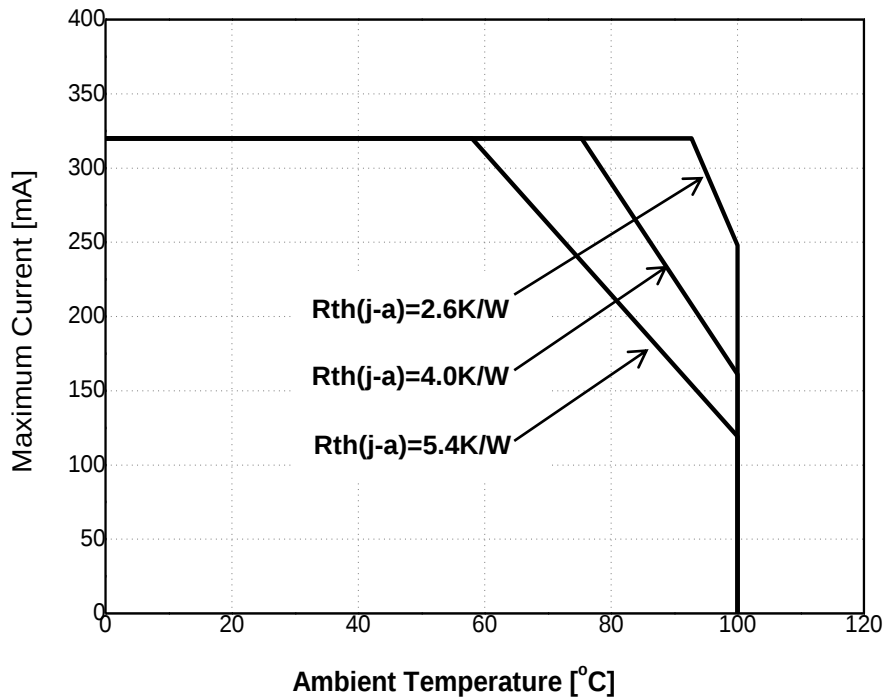
Fig 9. Maximum Forward Current vs. Ambient Temperature, T_j(\text{max.}) = 125^\circ\text{C} , I_F = 0.32\text{A}
