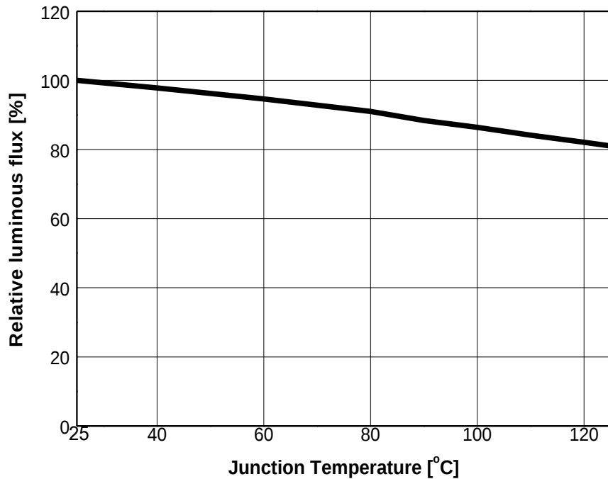
Fig 6. Relative Light Output vs. Junction Temperature, I_F = 180\text{mA}
