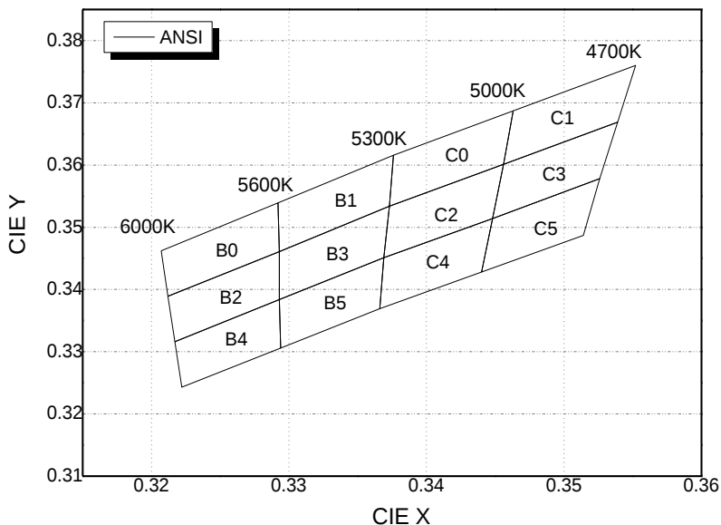
CIE Chromaticity Diagram (Cool white), Tc=25℃, IF=180mA
