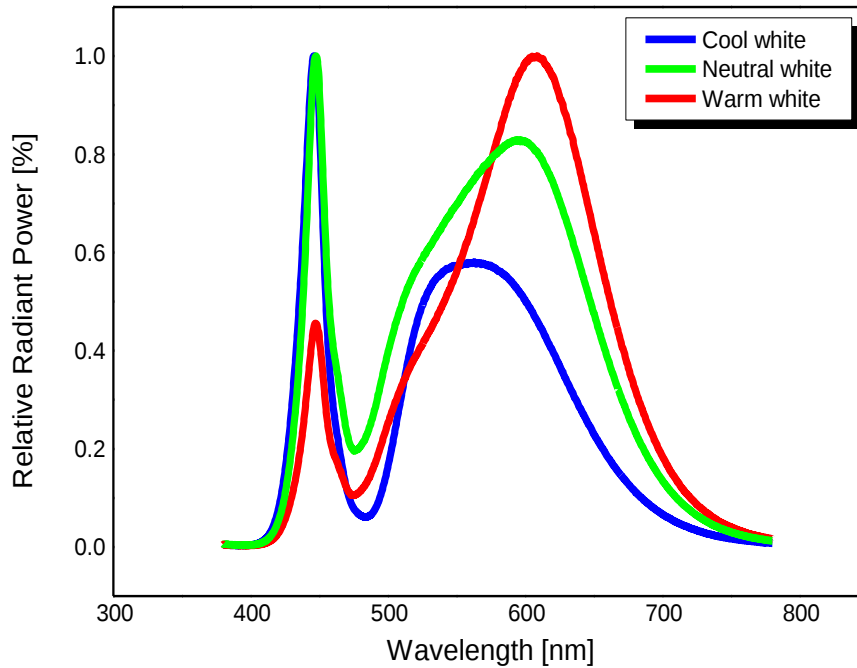
Fig 1. Color Spectrum, T_c = 25^\circ\text{C} , I_F = 180\text{mA} , RH30%
