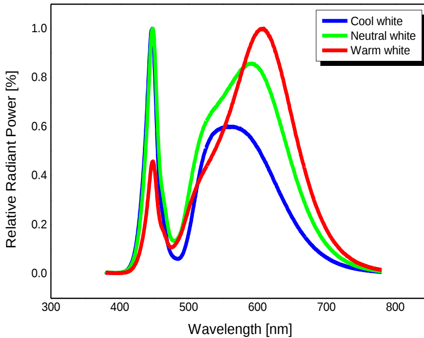
Fig 1. Color Spectrum, Ta = 25℃, IF = 700mA, RH30%
